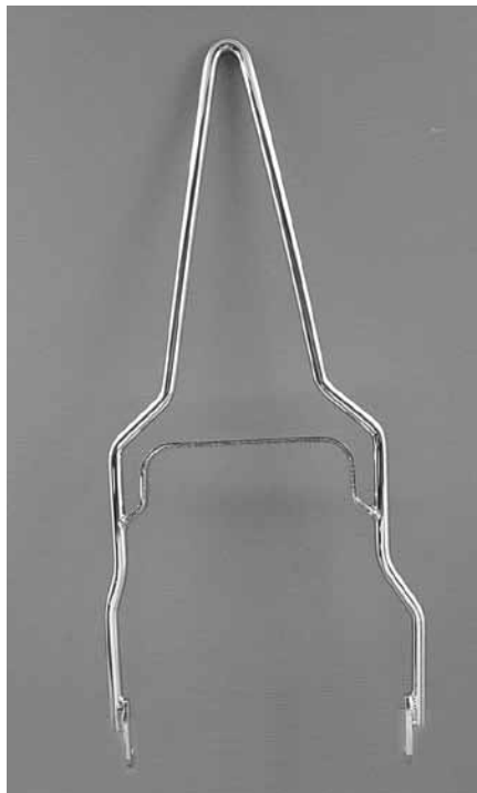
Chrome Round Sissy Bar Is constructed of 5/8" steel to fit 8-9" flat fender with belt drive. Height is 30". 55810
